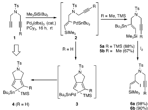
Scheme 1. Selectivity in the Silylstannylation of Acetylenes
