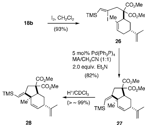
Scheme 2. Cyclopentane Annulation via Heck Reaction
